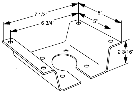
Style "C" Standard Base
